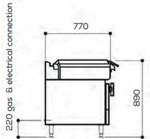
Unit on castors is same height
